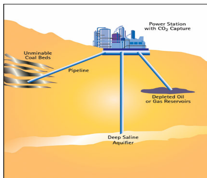
Figure 3. Geologic storage options (courtesy of the IEA Greenhouse Gas R&D Programme)
