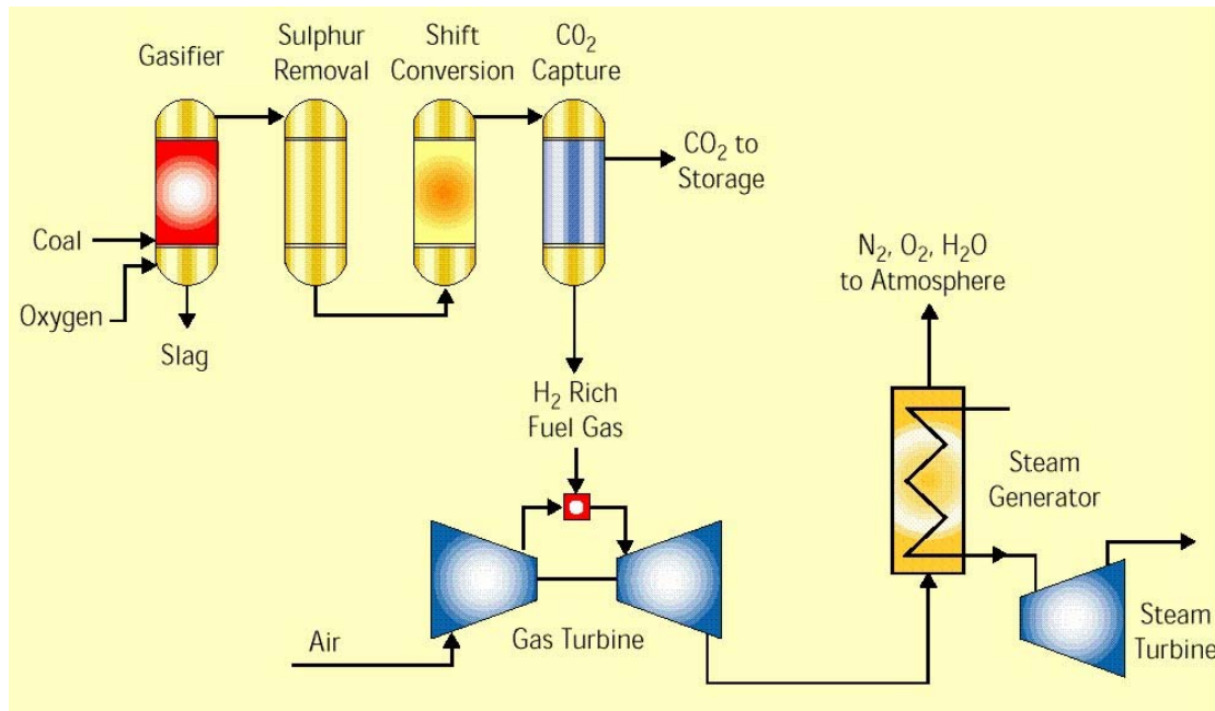
Figure 2. Coal-fired IGCC with pre-combustion capture of CO 2 (courtesy of the IEA Greenhouse Gas R&D Programme)
